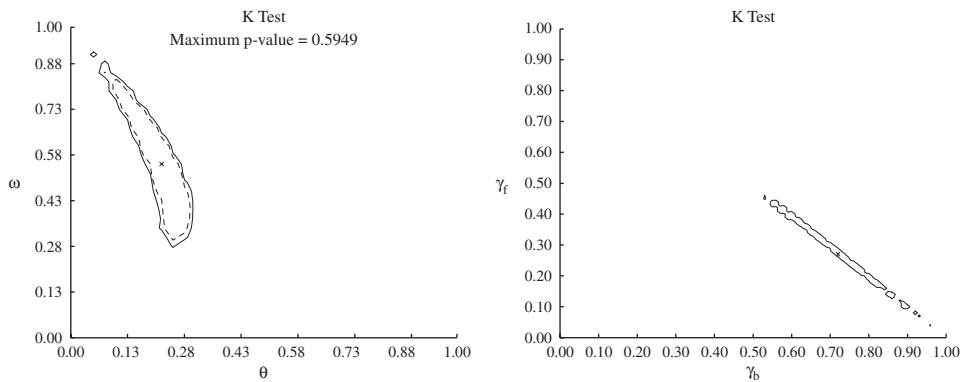
Fig. 2. AR-K tests (U.S., survey expectations).
