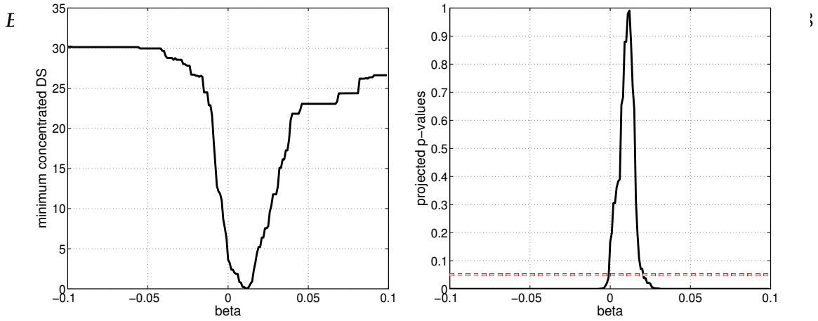
Figure 5. Concentrated statistics and projected p -values (1880-1930)
